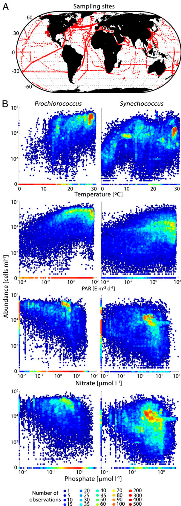
Fig. 1. Observations of Prochlorococcus and Synechococcus cell abundance. (A) Geographic distribution of samples used in this study. (B) Prochlorococcus and Synechococcus as a function of temperature, PAR, nitrate, and phosphate concentration. Symbol color represents the number of overlapping observations.
