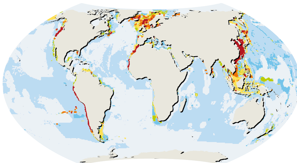
Figure 20: The world's most productive fishing grounds are confined to major hotspots in around 7.5% of the ocean surface, where over half of the fish are caught.
