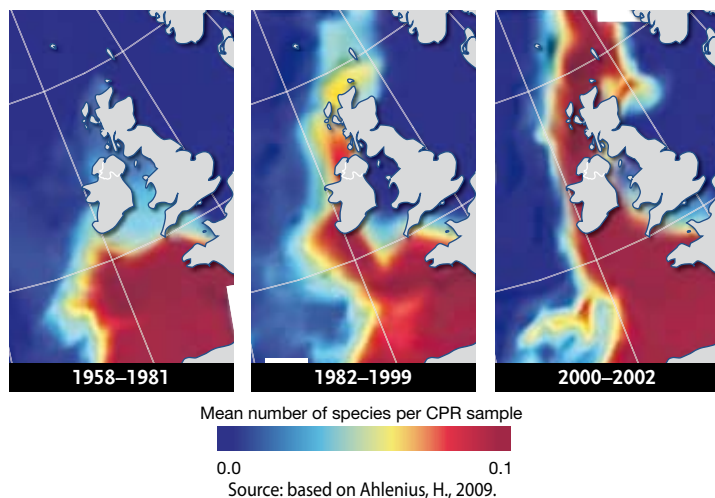
Figure 13. Plankton migration shift.
